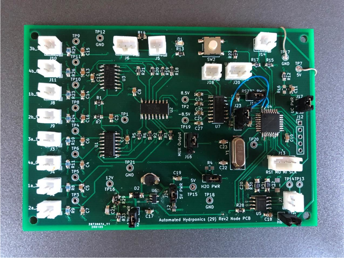
Node PCB
