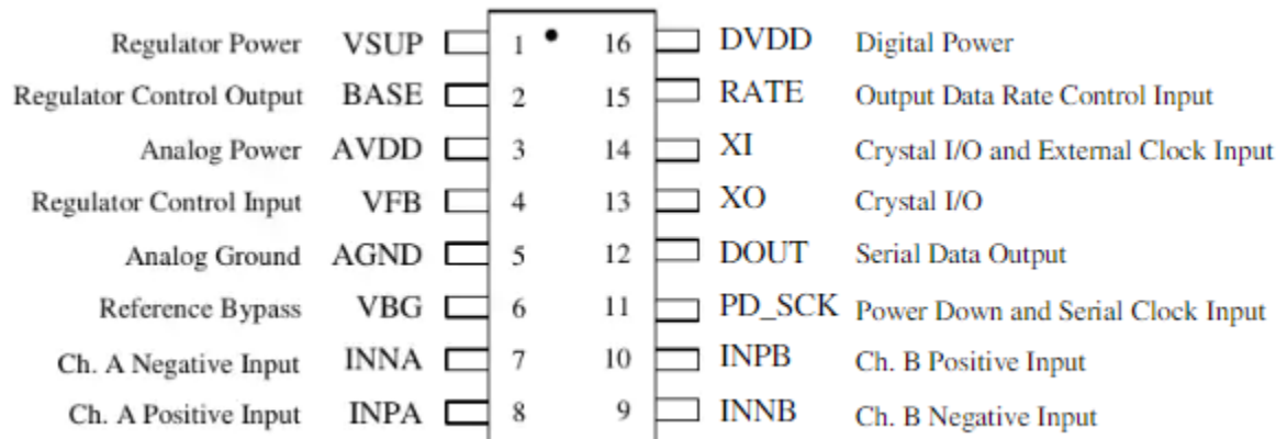
Fig. 2. HX711 Pin Layout
