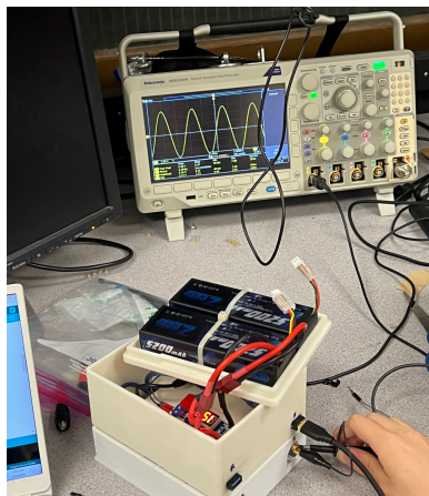
i) Measurement setup
